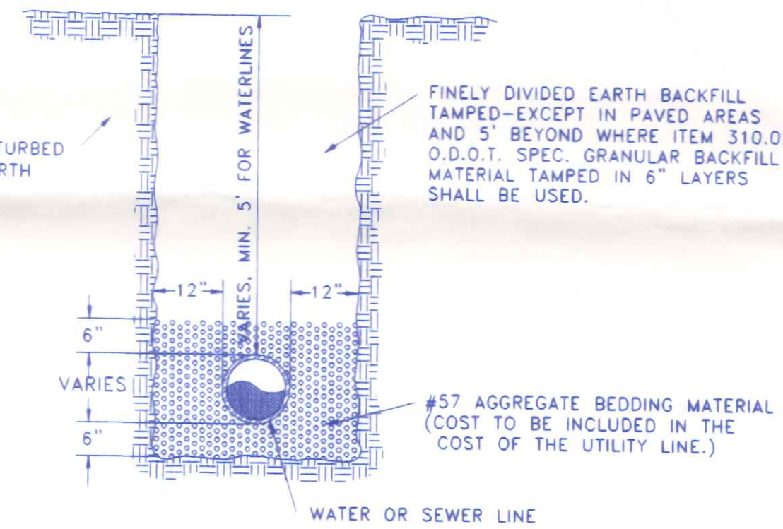
TYPICAL UTILITY LINE TRENCH DETAIL SCALE: 1/2" = 1'-0"
