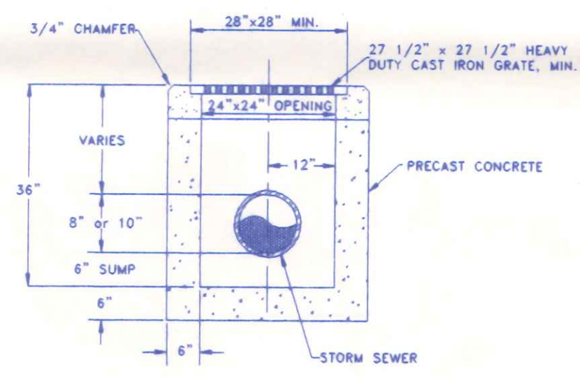
RELOCATED CATCH BASIN DETAIL SCALE: 1/2" = 1'-0"
