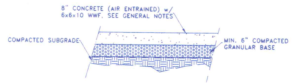
TYPICAL CONCRETE PAVEMENT SECTION SCALE: 1/2" = 1'-0"
