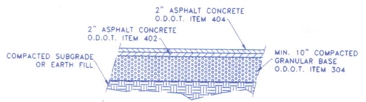
TYPICAL ASPHALT PAVEMENT SECTION SCALE: 1/2" = 1'-0"
